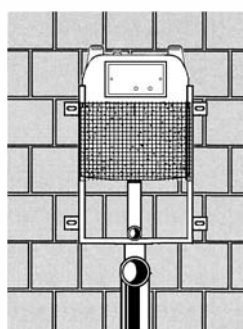
FRONTE PARETE Wall face
