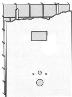
INCASSO A MURARE Built-in in brickwork
