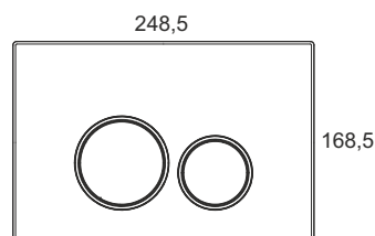
Cod. CPLSTYLE5
